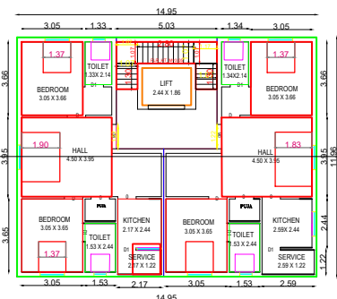
FIRST FLOOR PLAN TYPICAL_FLOOR_PLAN=1,2,3
