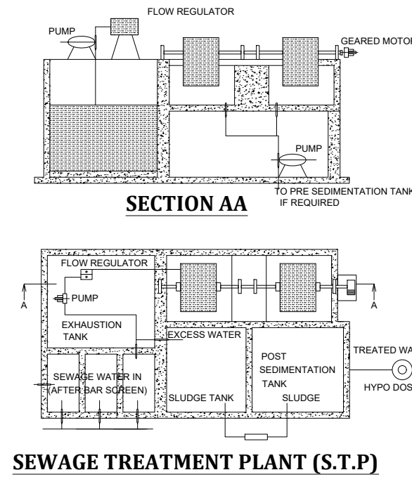
SEWAGE TREATMENT PLANT (S.T.P)
