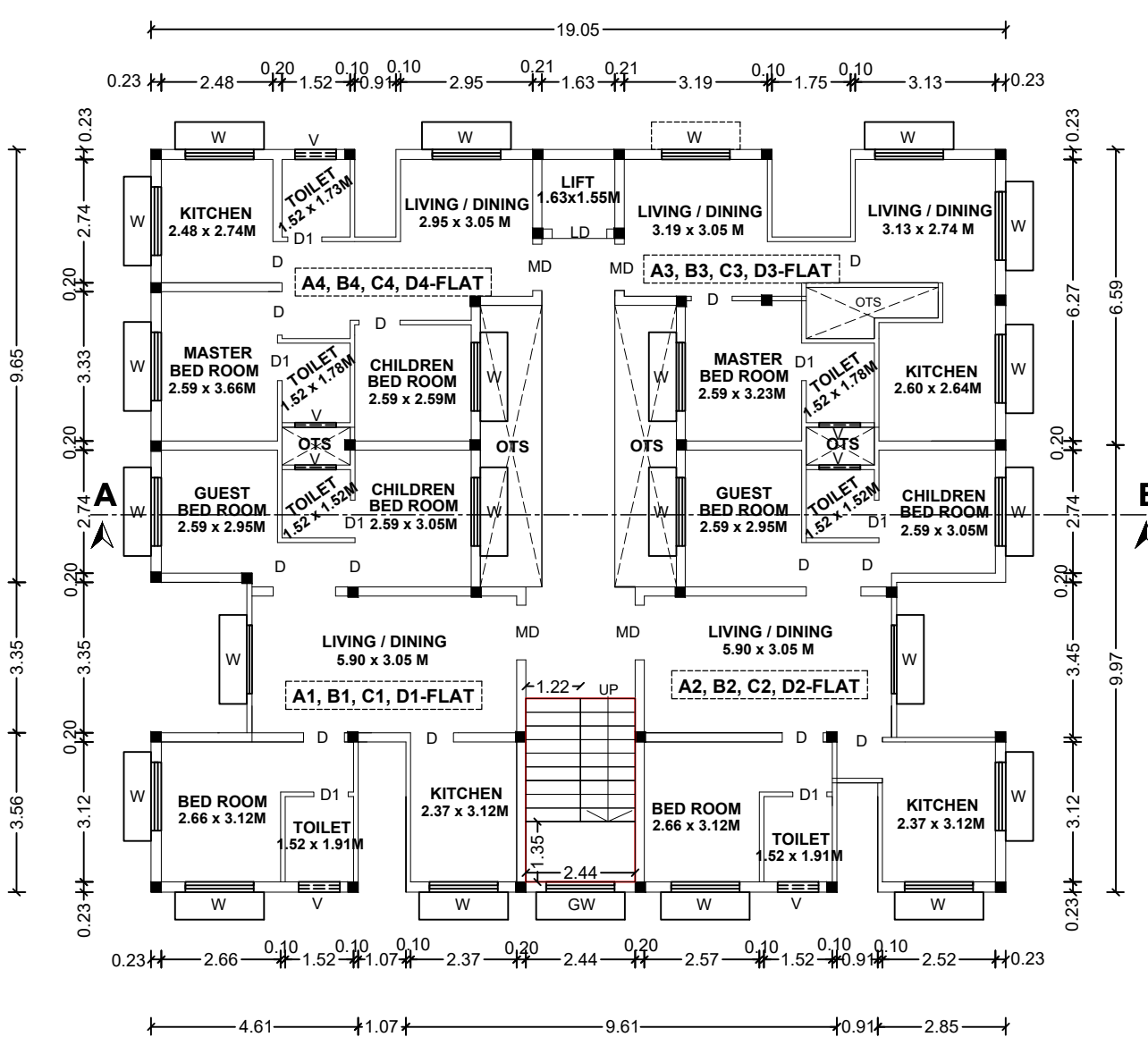
TYPICAL FIRST, SECOND, THIRD & FOURTH FLOOR PLAN
