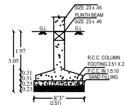
FOUNDATION DETAIL (DETAIL - B)
