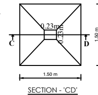
SECTION - 'CD'
