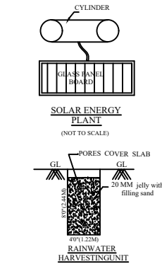
RAINWATER HARVESTING UNIT
