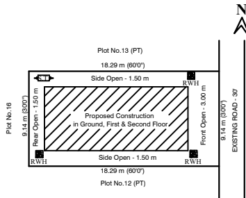
SITE PLAN
