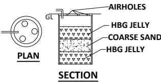
RAIN WATER HARVESTING UNIT
