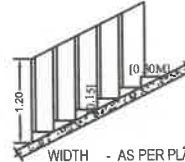
STAIRCASE DETAILS
