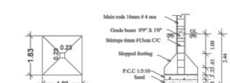
FOOTING / COLUMN DETAIL
