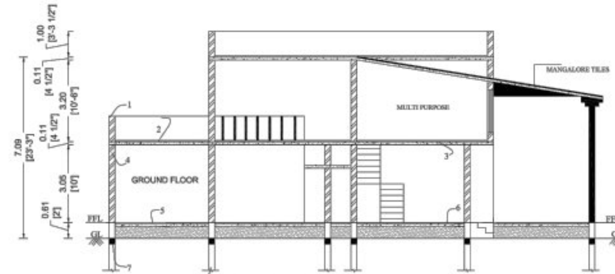
SECTION ON "JS"
