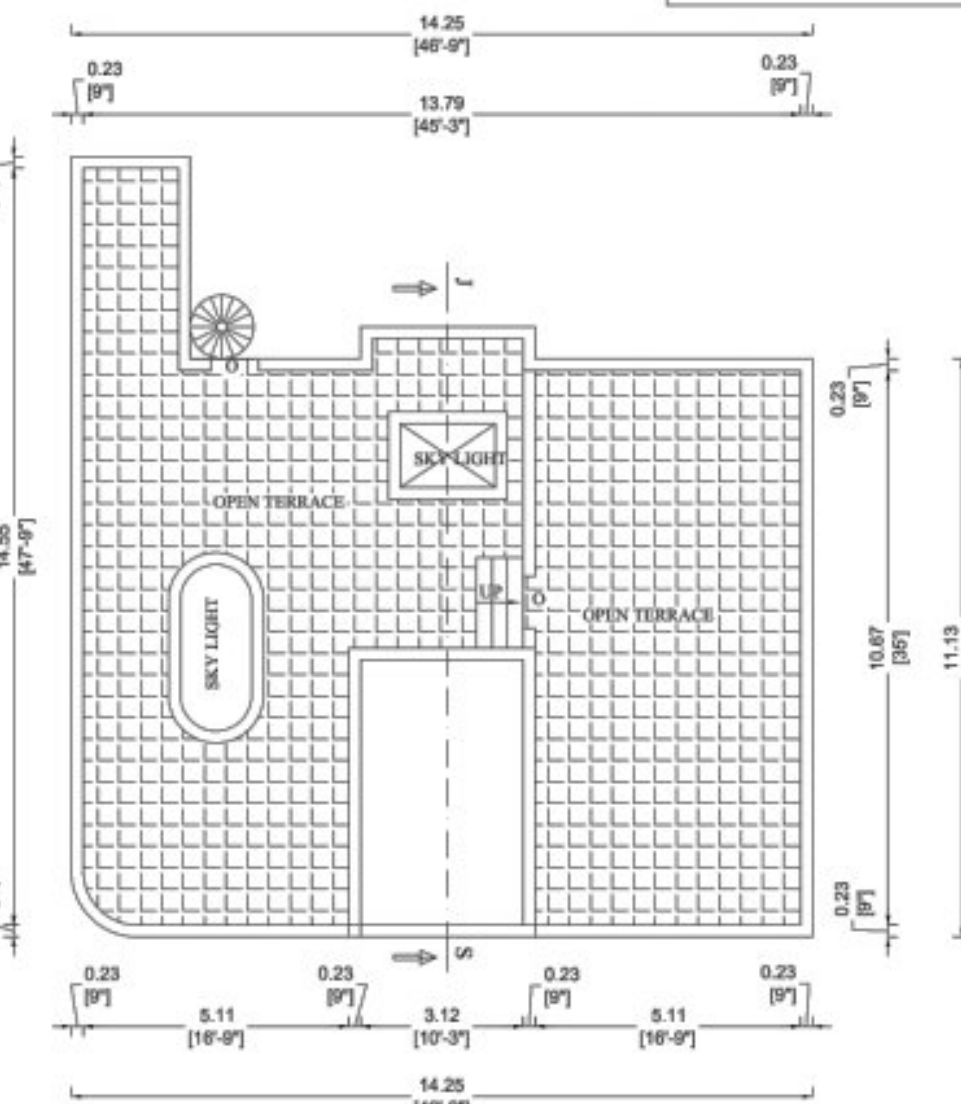
PRO., OPEN TERRACE FLOOR PLAN
