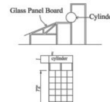
SOLAR ENERGY SYSTEM
