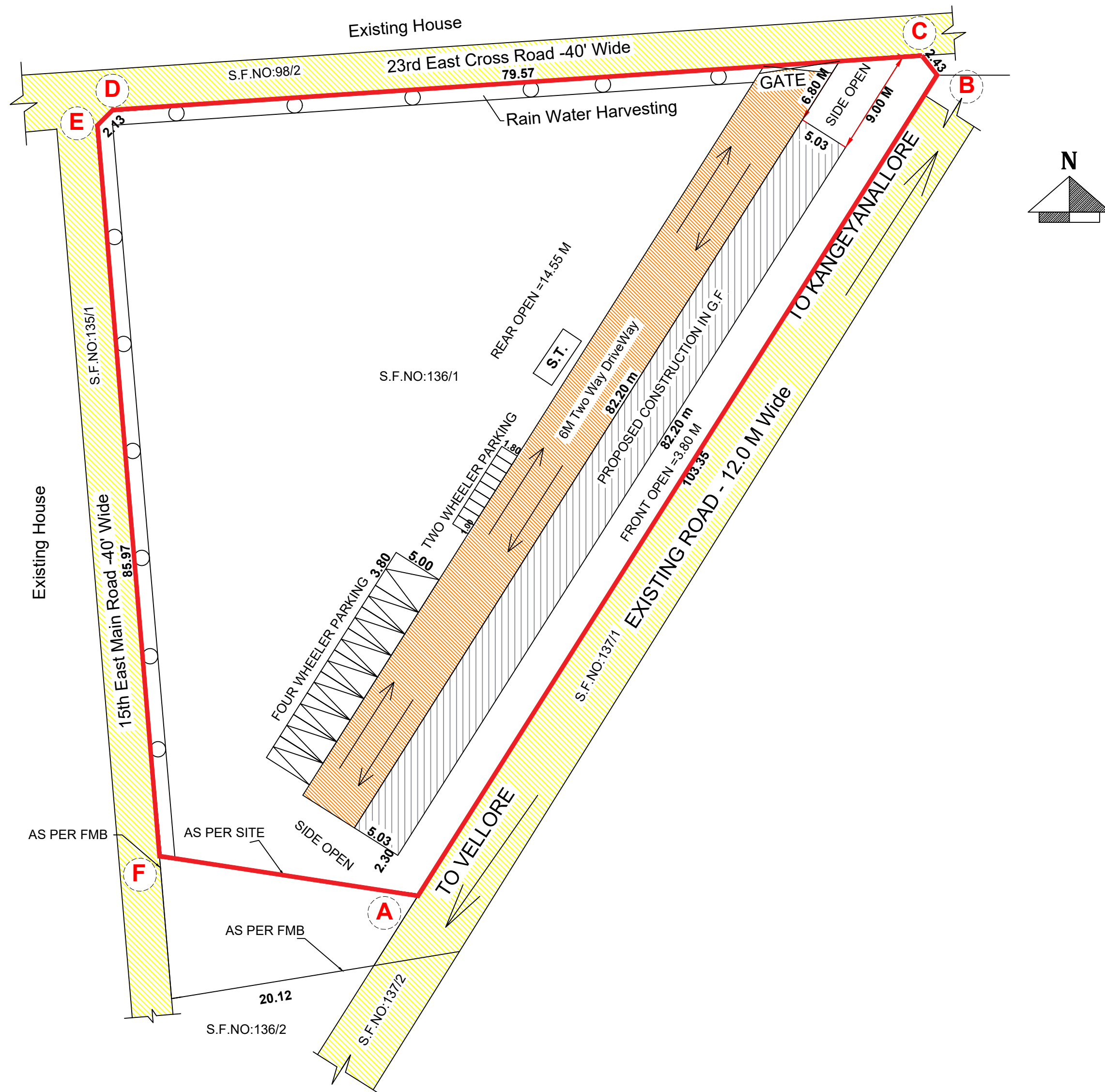
SITE PLAN
