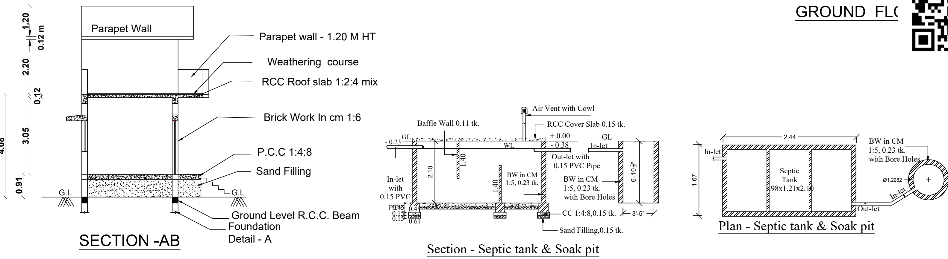
SECTION - Septic tank & Soak pit
