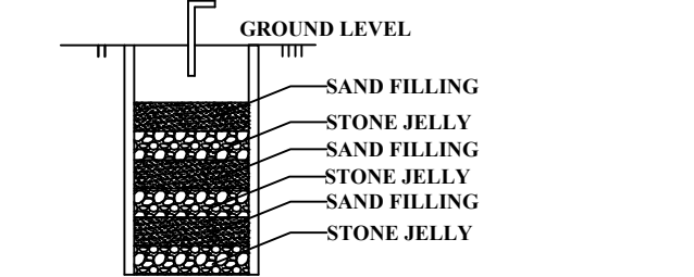
RAIN WATER HARVESTING TANK
