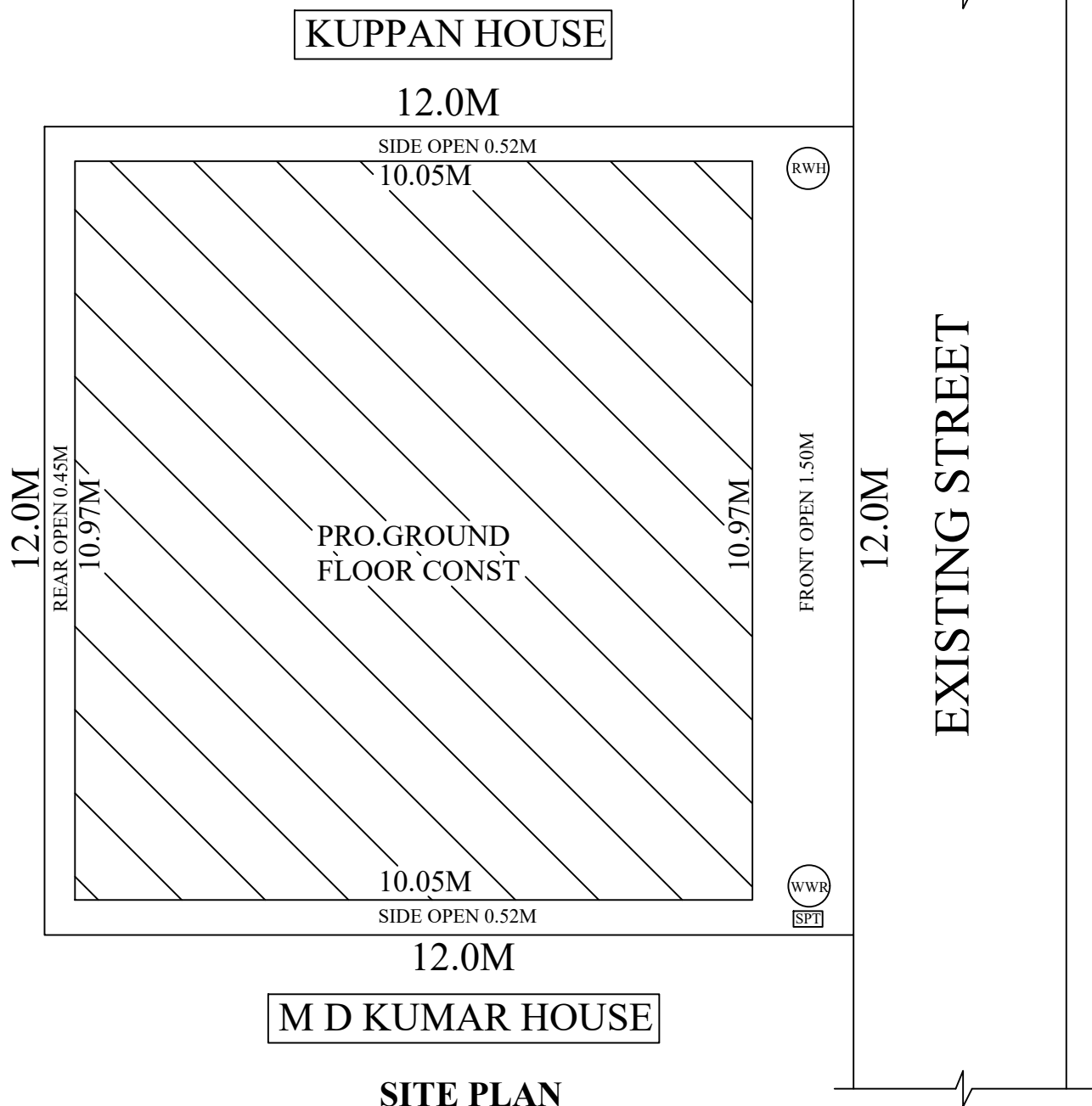
SITE PLAN
