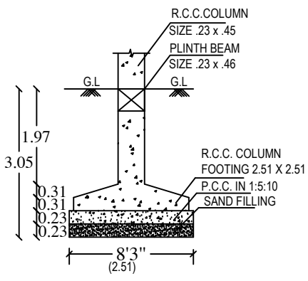
FOUNDATION DETAIL
