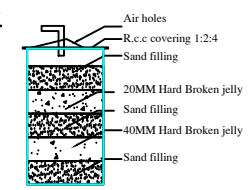
RAIN WATER UNITS
