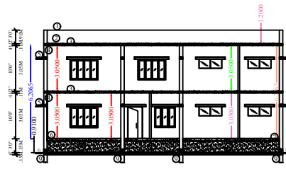
SECTION ON 'CY'
