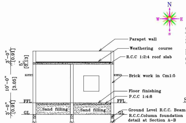
SECTION ON 'SS'
