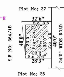
SITE PLAN SCALE: 1INCH=33FEET
