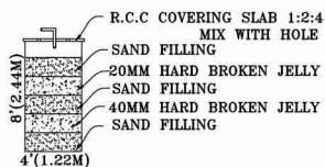
RAIN WATER HARVEST UNIT
