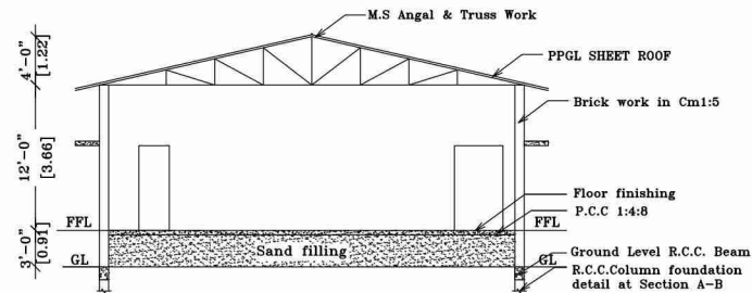
SECTION ON 'SS'
