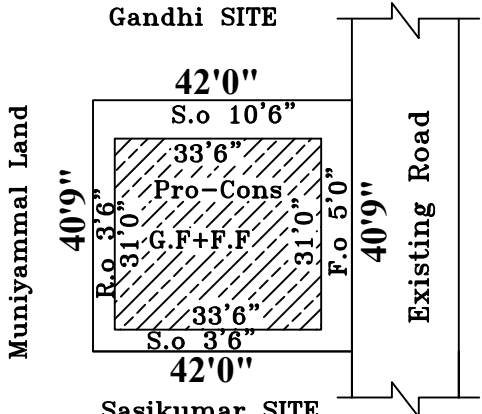
SITE PLAN SCALE: 1INCH=33FEET
