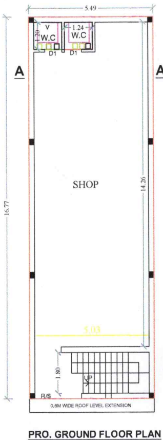
PRO. GROUND FLOOR PLAN
