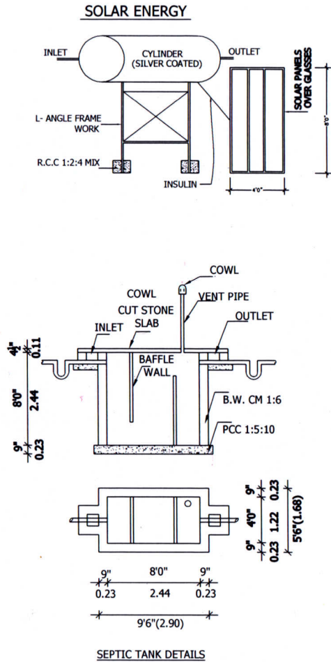
SEPTIC TANK DETAILS
