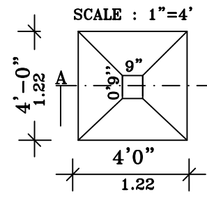
COLUMN DETAILS
