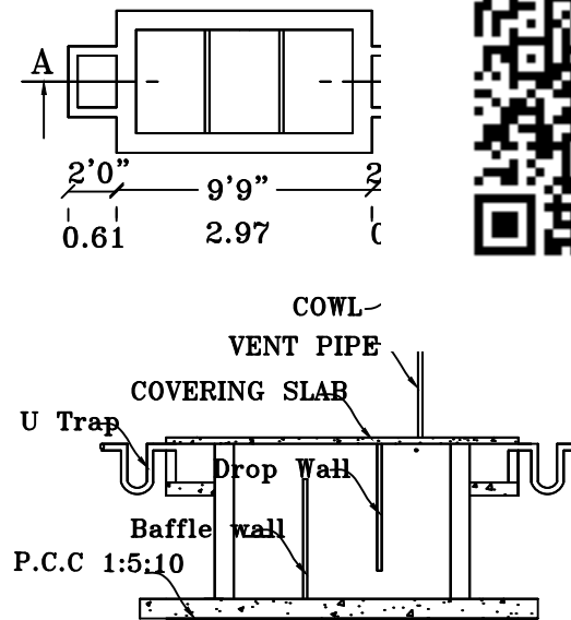
SEPTIC TANK I
