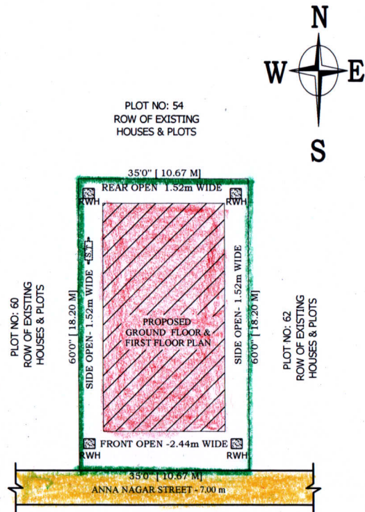
SITE PLAN
