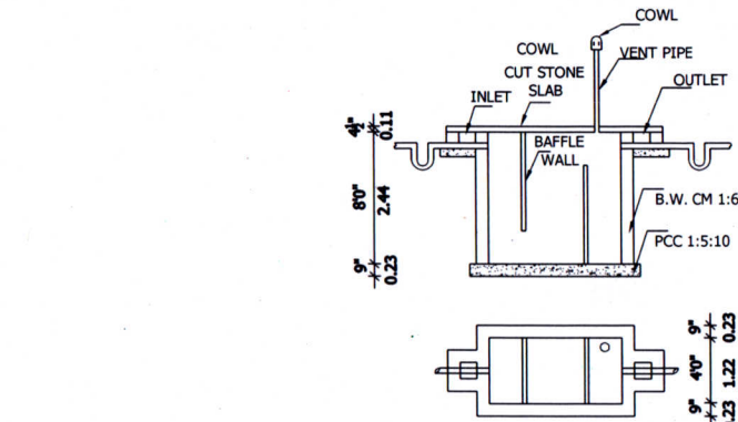
WASTE WATER RECYCLE UNIT
