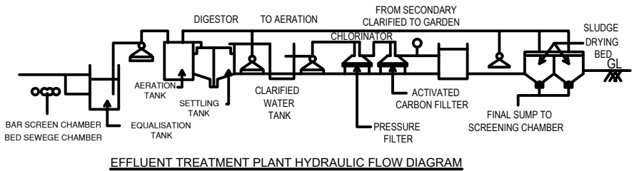
EFFLUENT TREATMENT PLANT HYDRAULIC FLOW DIAGRAM
