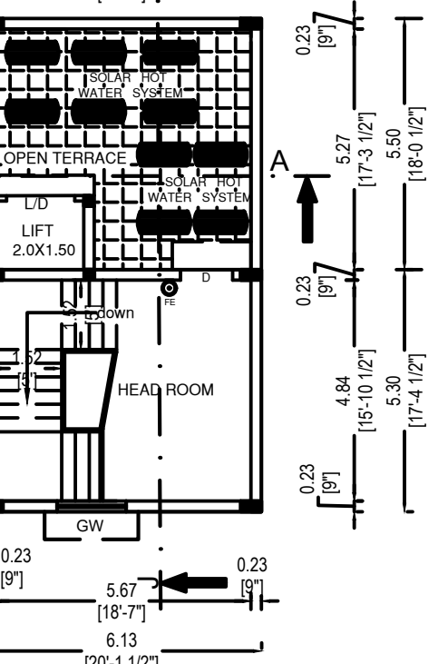
OPEN TERRACE FLOOR PLAN
