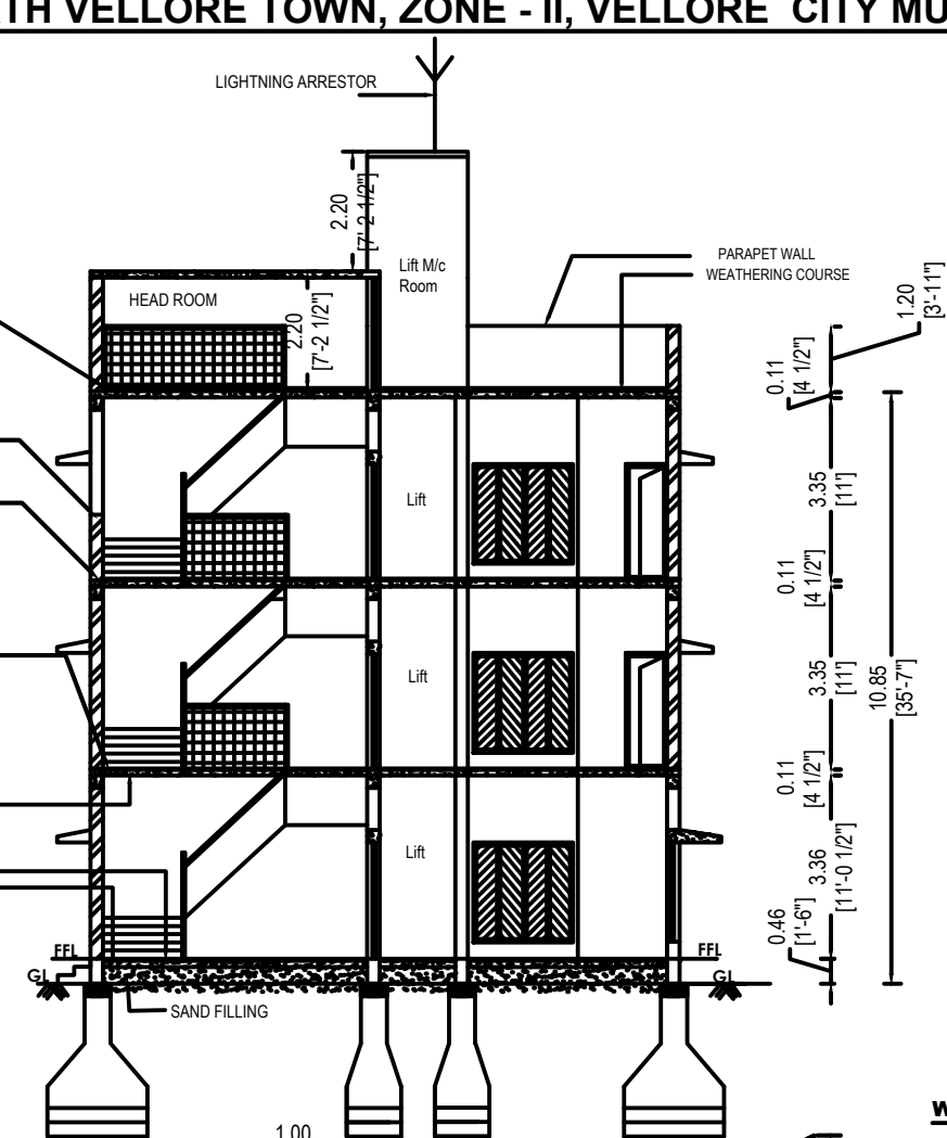
SECTION ON "JS"
