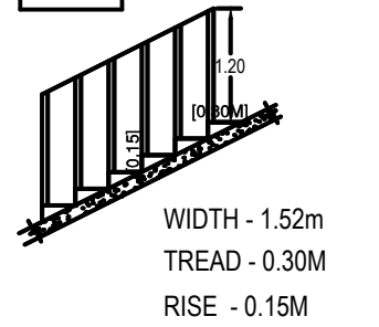
STAIRCASE DETAILS
