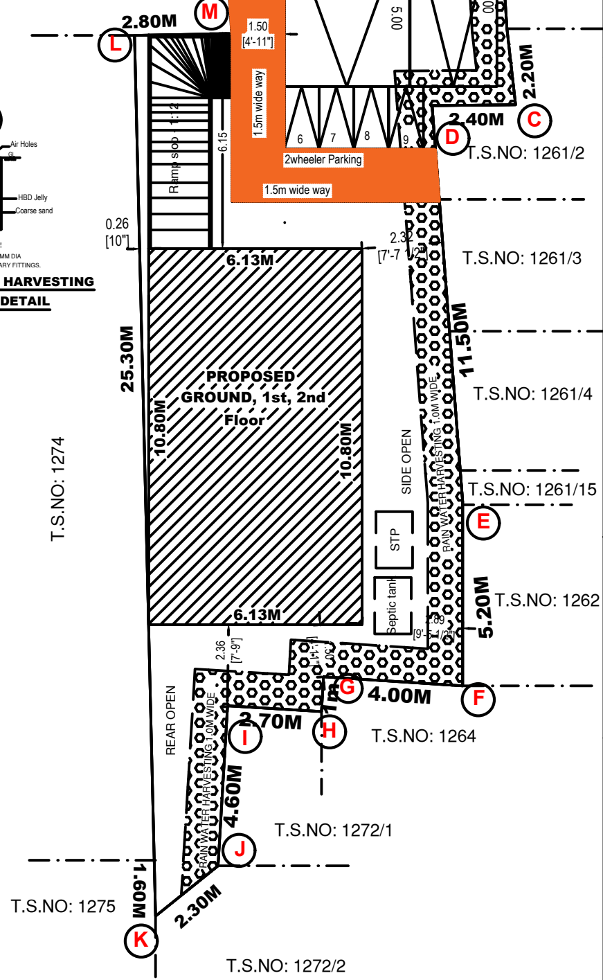
SITE PLAN
