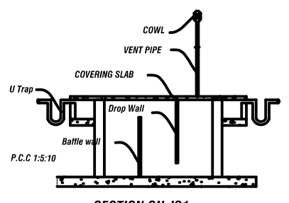
SECTION ON JS1
