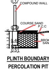
PLINTH BOUNDARY PERCOLATION PIT
