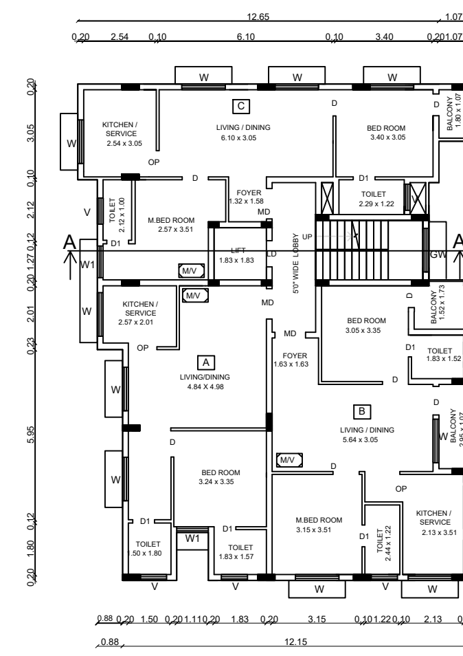
TYPICAL SECOND, THIRD & FOURTH FLOOR PLAN
