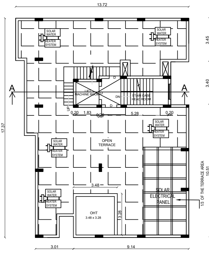
OPEN TERRACE FLOOR PLAN
