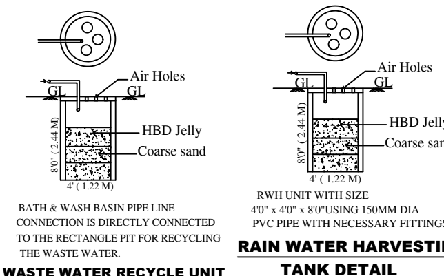
WASTE WATER RECYCLE UNIT
