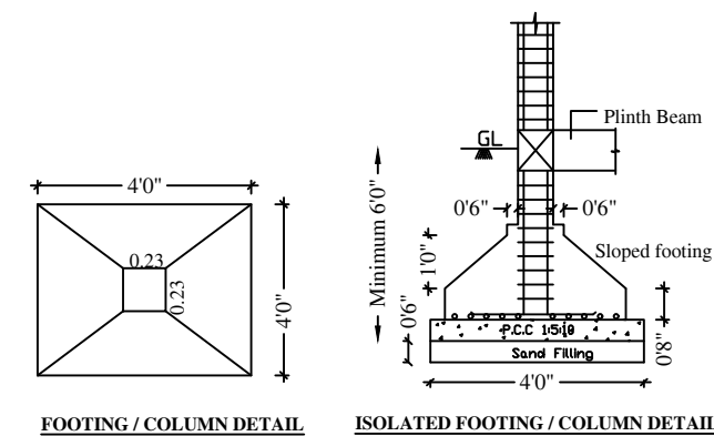
COLUMN DETAILS
