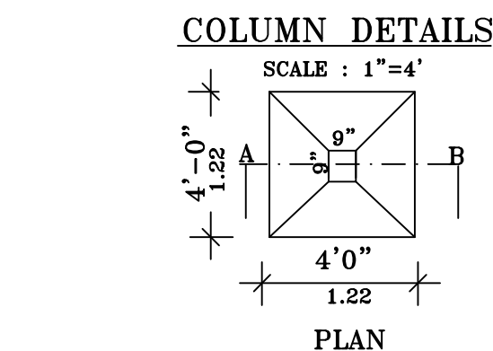
Main rods 16mm# 4nos Grade beam 0'9"x1'3" Stirrups 6mm#15cmC/C Sloped footing P.C.C 1:5:10 Sand Filling 4'0" 1.22 SECTION ON A-B
