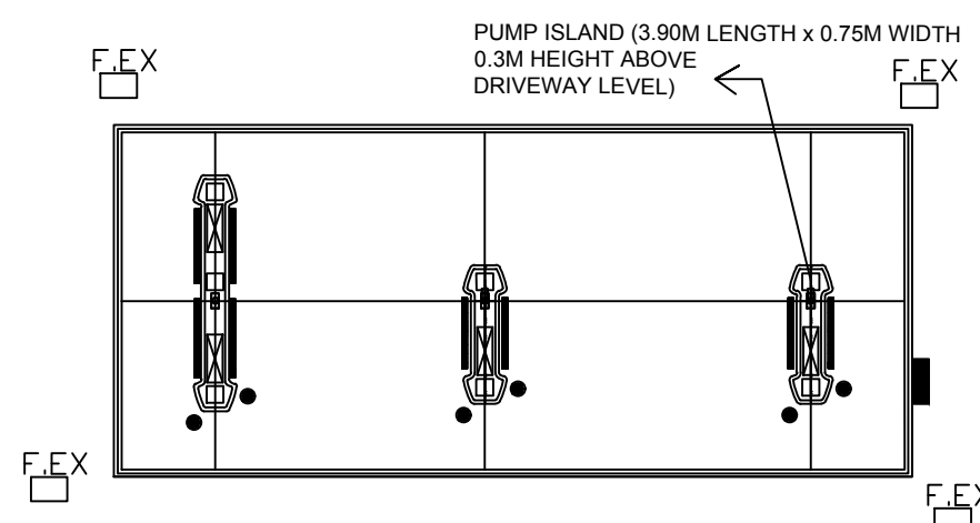
CANOPY PLAN
