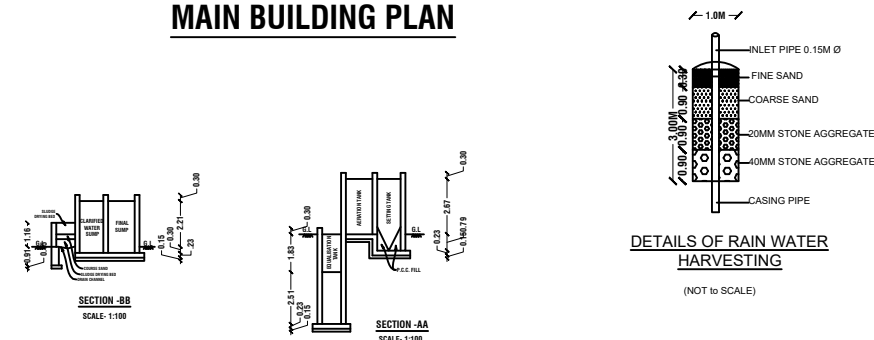
MAIN BUILDING PLAN
