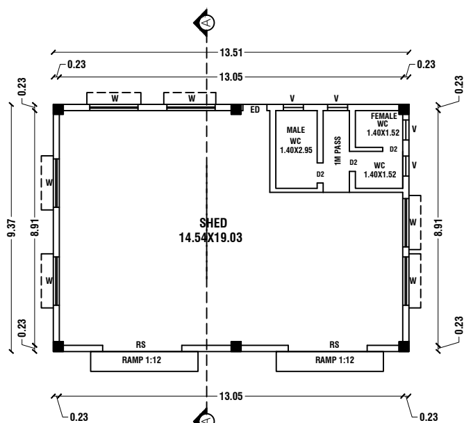
MAIN BUILDING PLAN
