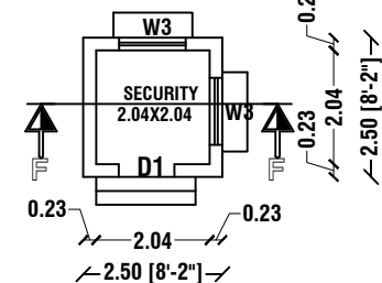
SECURITY OFFICE PLAN
