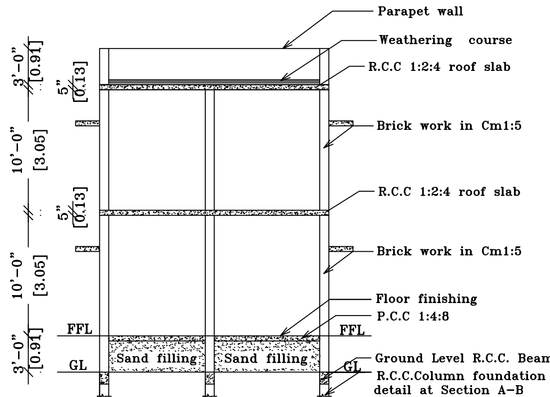
SECTION ON 'SK'
