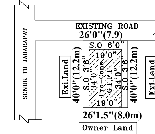
SITE PLAN
