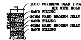
RAIN WATER HARVEST UNIT
