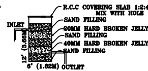
WASTE WATER RECYCLE UNIT
