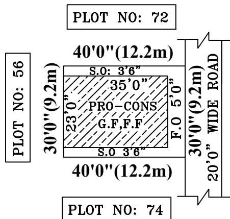
SITE PLAN
