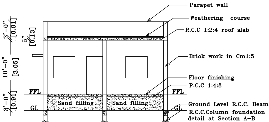
SECTION ON 'SS'
