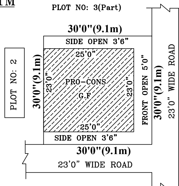
SITE PLAN
