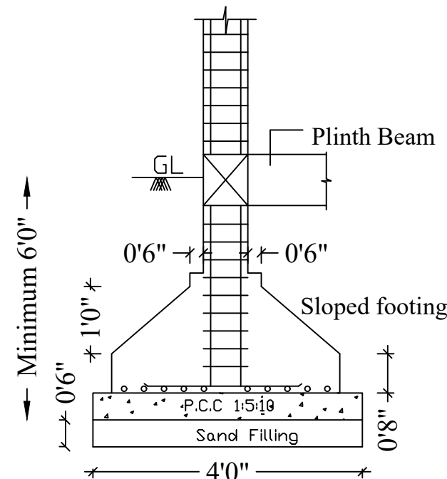
ISOLATED FOOTING / COLUMN DETAIL
