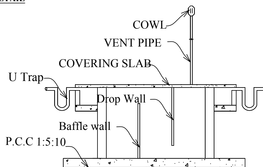
SECTION ON JS1
