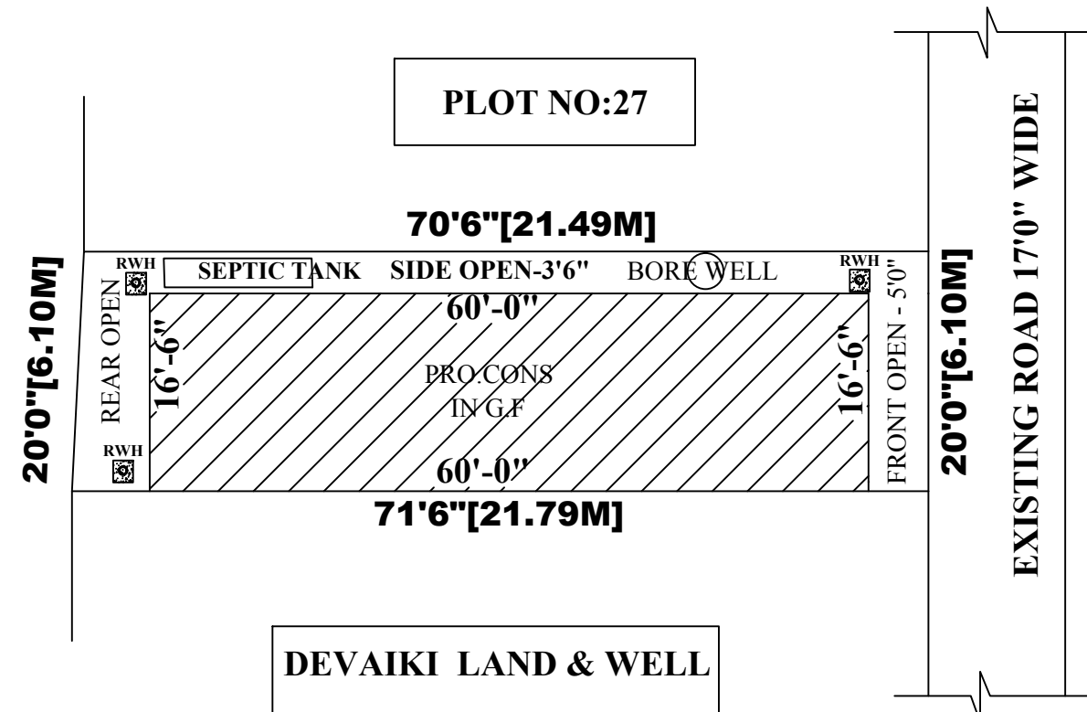
SITE PLAN
