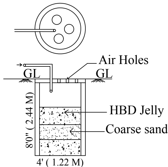
RAIN WATER HARVESTING TANK DETAIL
