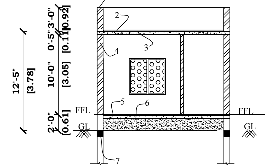
SECTION ON "JS"
