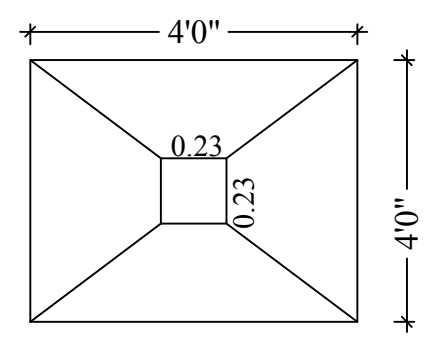
FOOTING / COLUMN DETAIL
