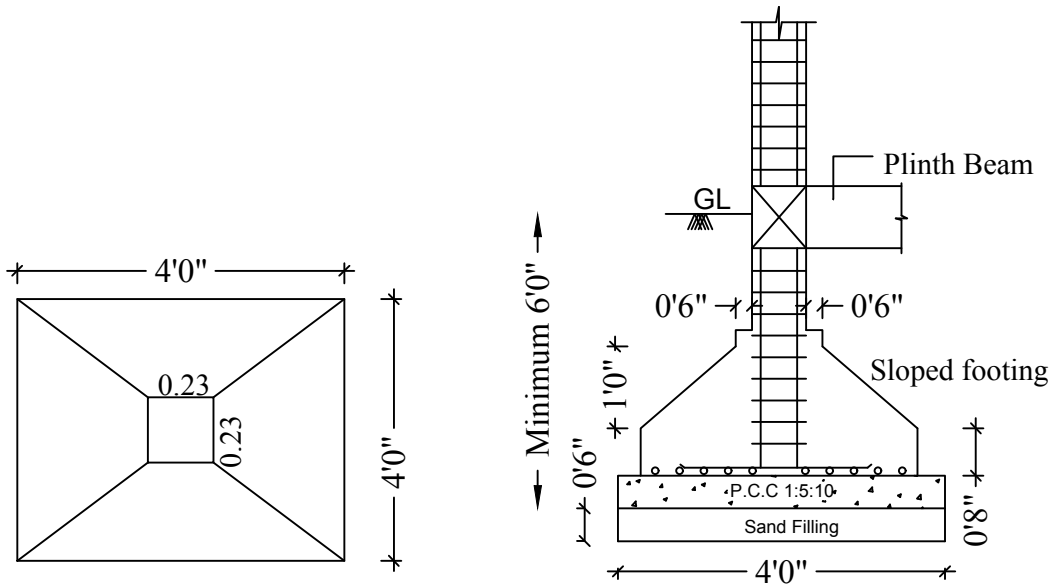
FOOTING / COLUMN DETAIL
