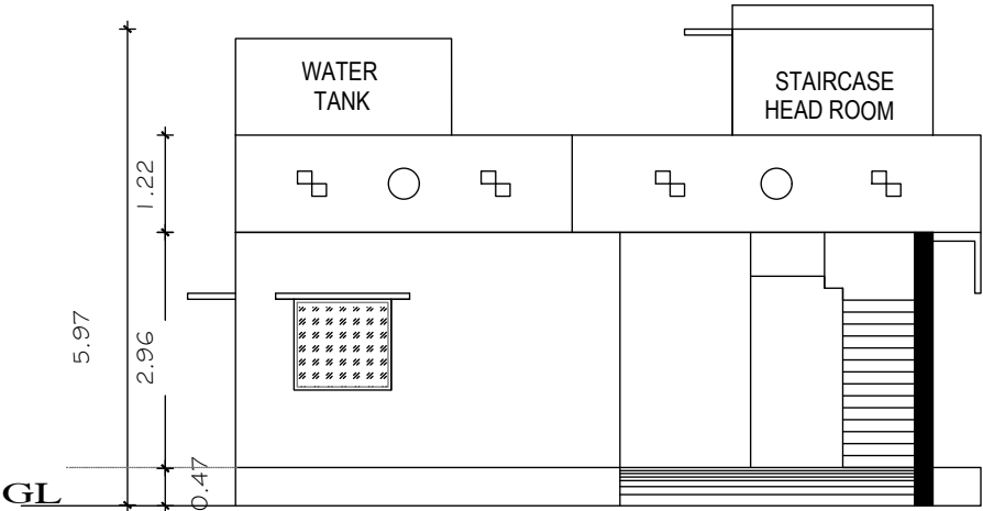
FRONT ELEVATION.
