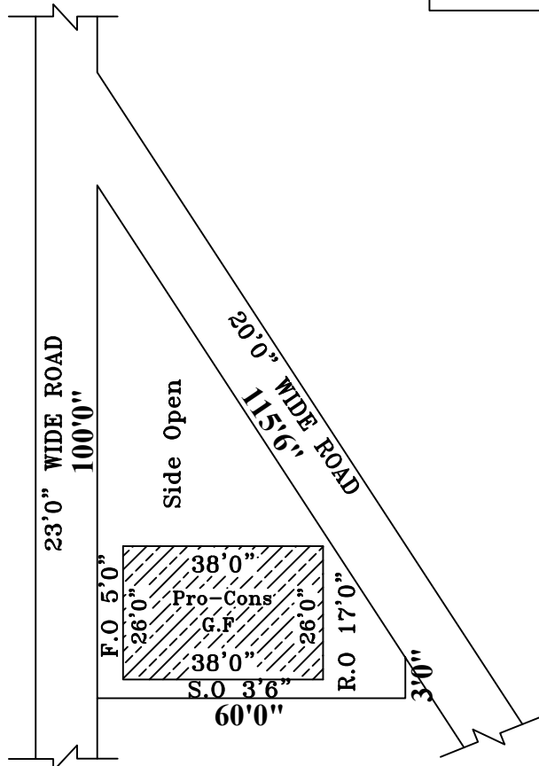
SITE PLAN
