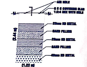
RAINWATER HARVESTING UNIT RWHT - SIZE: 1.22 X 1.22 X 2.44 - 2 NOS USING 150MM PIPE AND NECESSARY SPECIALS. SCALE: 1:50
