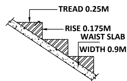
SECTION OF THE STAIRCASE NOT TO SCALE
