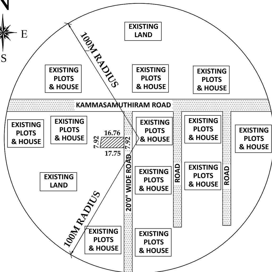
TOPOGRAPHY PLAN - FOR 100M RADIUS
