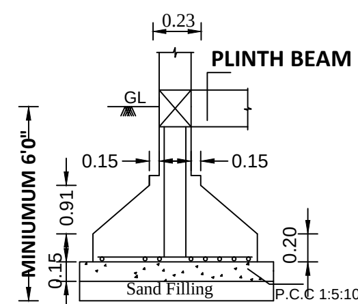
ISOLATED FOOTING (5'0"X5'0")
