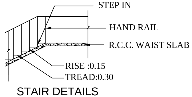
STAIR DETAILS
