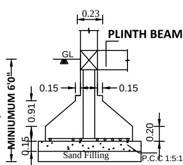
ISOLATED FOOTING (5'0"X5'0")
