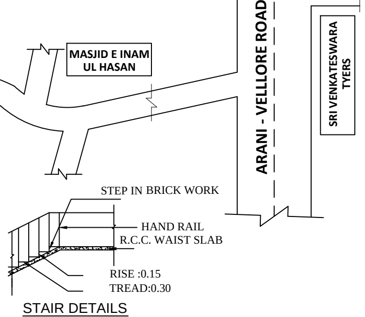
STAIR DETAILS
