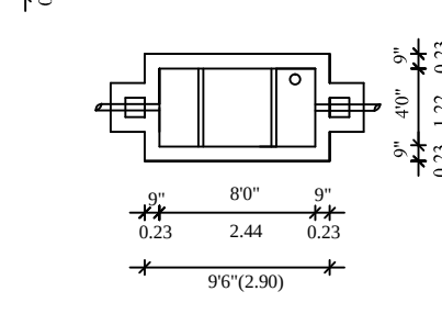
RAIN WATER HARVESTING SUMP (Scientificallly Closed)
