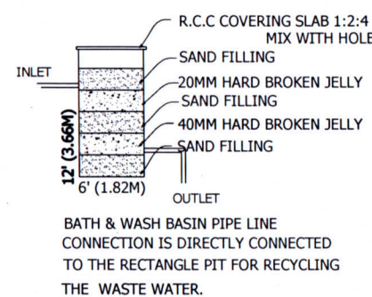
WASTE WATER RECYCLE UNIT
