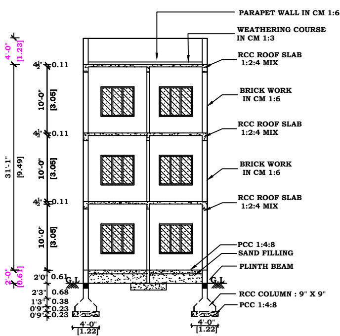
SECTION - KK
