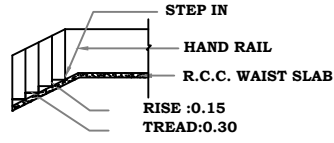
STAIR DETAILS
