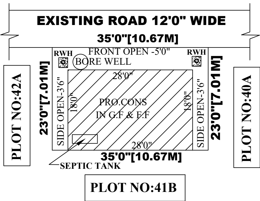
SITE PLAN
