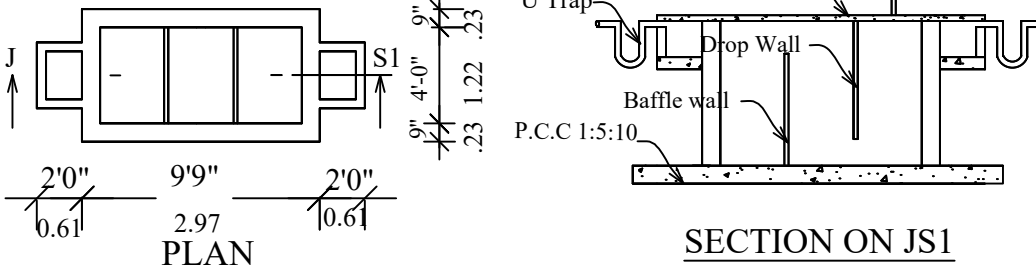
SEPTIC TANK DETAILS
