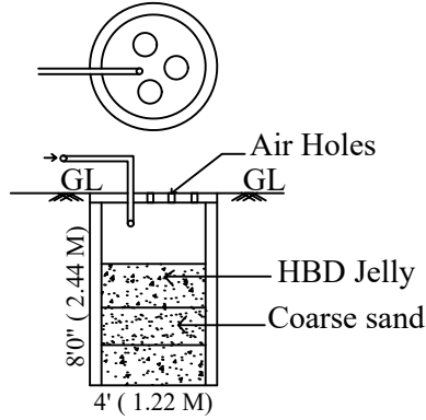
RAIN WATER HARVESTING TANK DETAIL
