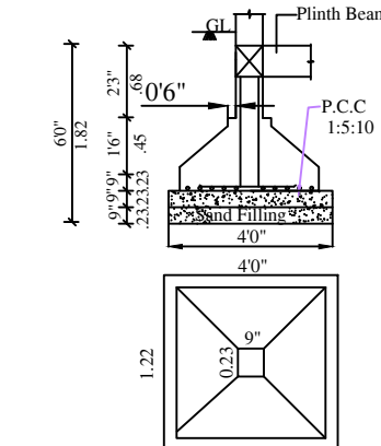
COLUMN DETAIL NOT TO SCALE
