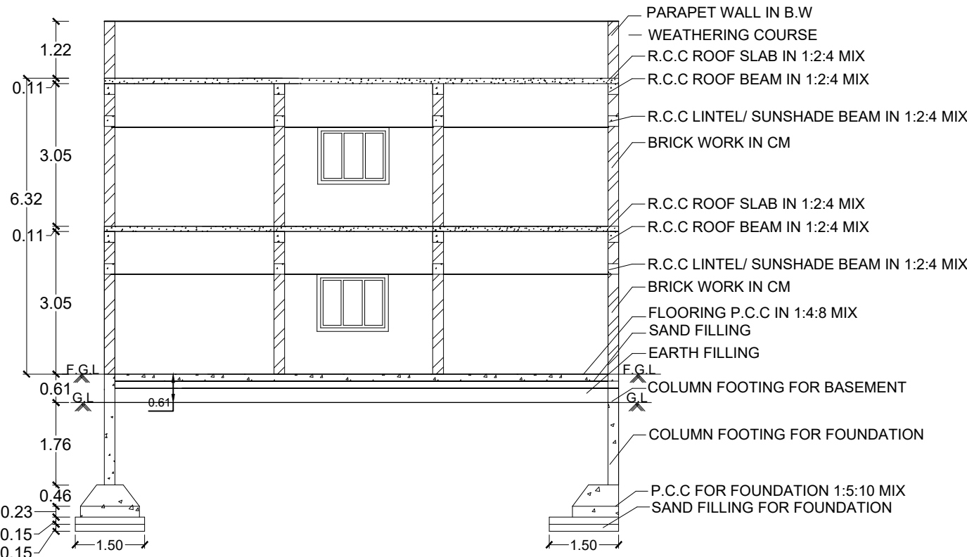
SECTION ON-AA
