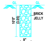
PERCOLATION PIT
