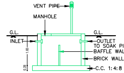
SECTION OF SEPT. TANK
