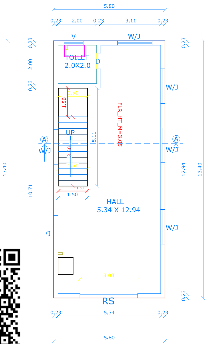
PRO.GROUND FLOOR
