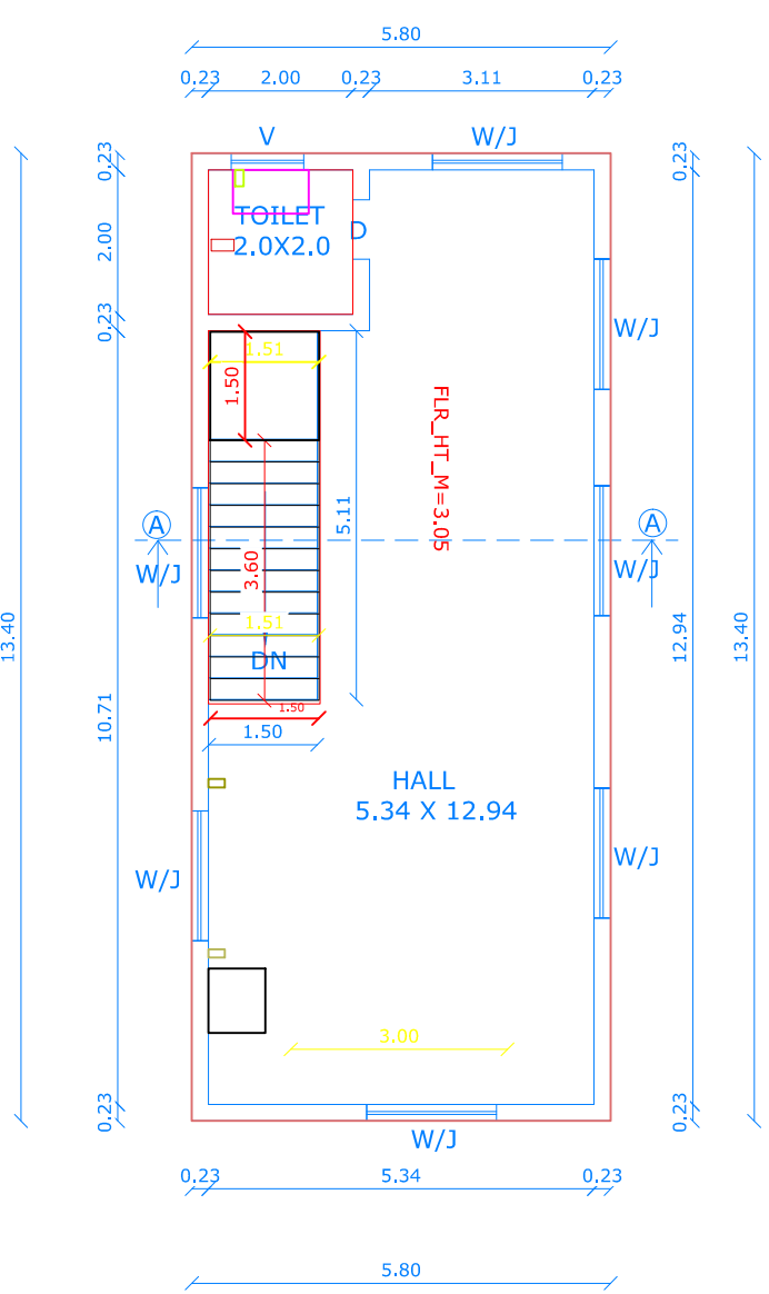
PRO.FIRST FLOOR
