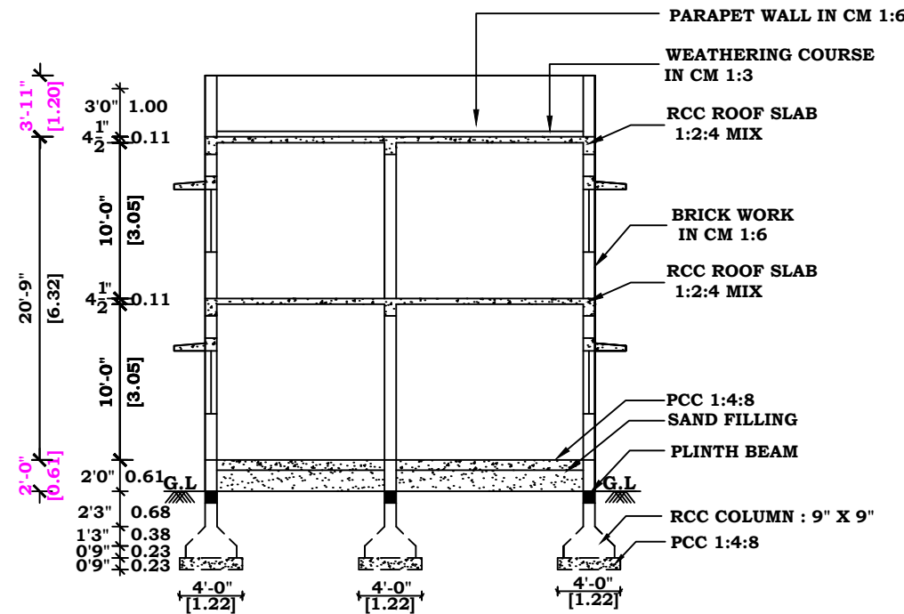
SECTION - KK
