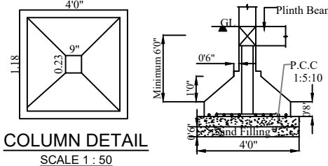
COLUMN DETAIL SCALE 1:50
