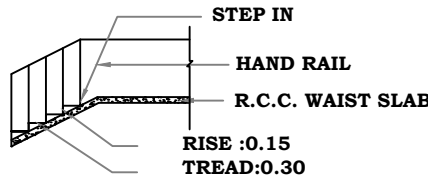
STAIR DETAILS
