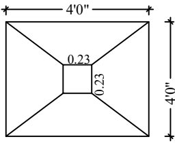
FOOTING / COLUMN DETAIL
