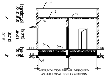
SECTION ON "JS"
