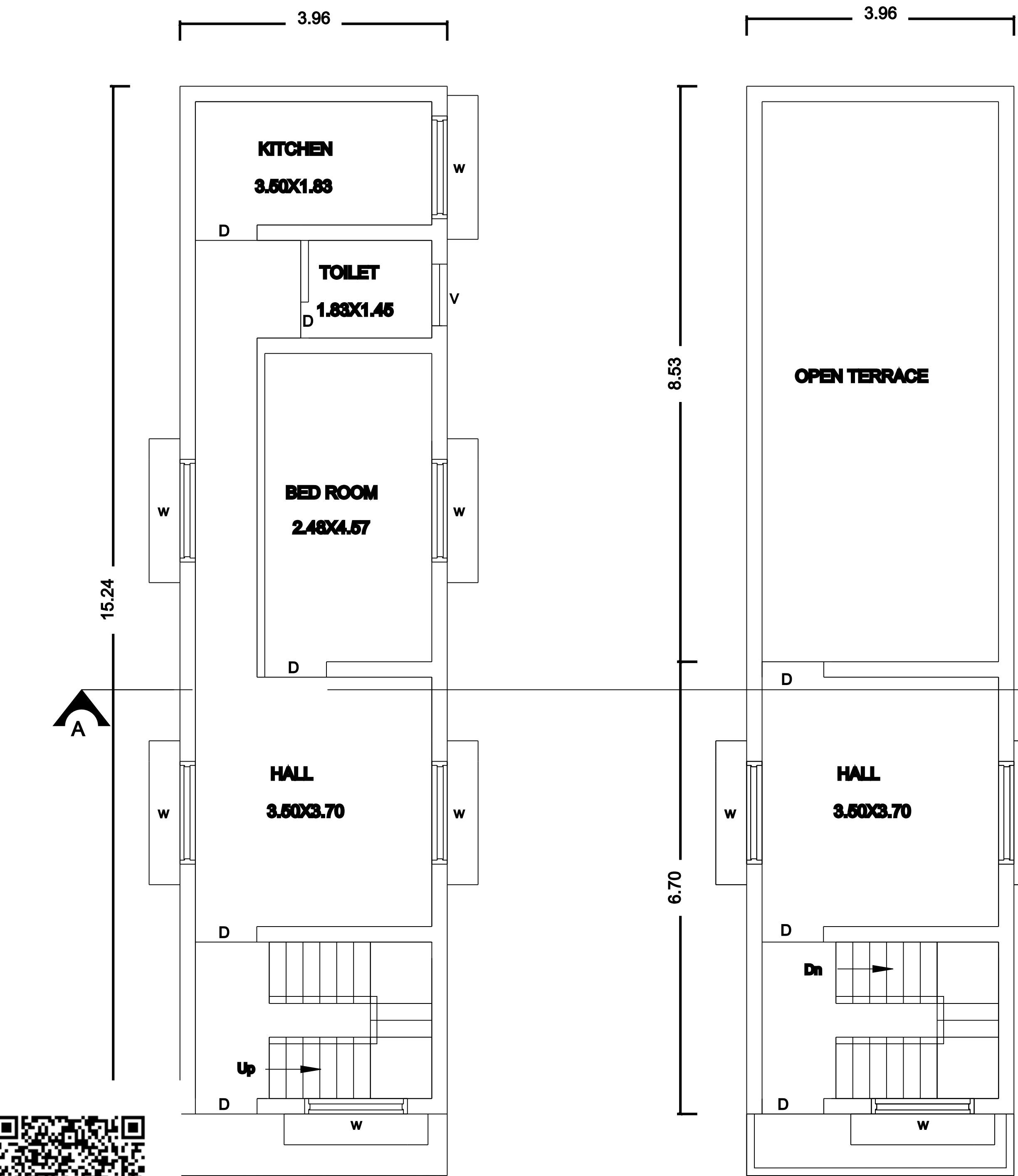
ND FLOOR PLAN
