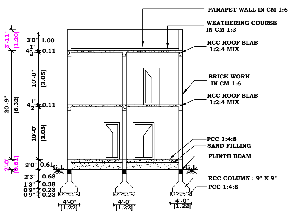
SECTION - KK
