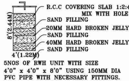
RAIN WATER HARVEST UNIT
