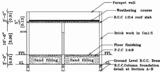
SECTION ON 'SA'
