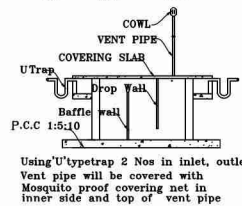
WASTE WATER RECYCLE UNIT
