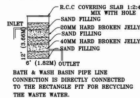
WASTE WATER RECYCLE UNIT
