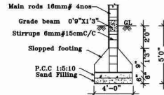
SECTION ON A-B
