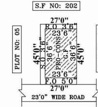
SITE PLAN
