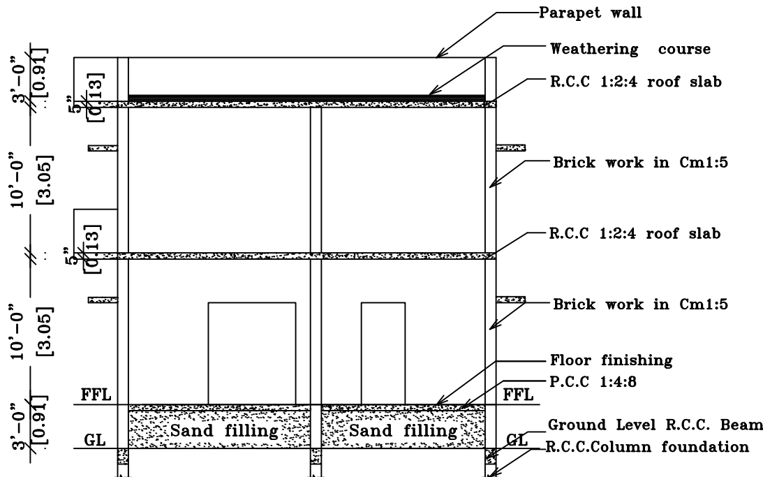
SECTION ON 'SK'
