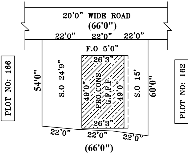
SITE PLAN
