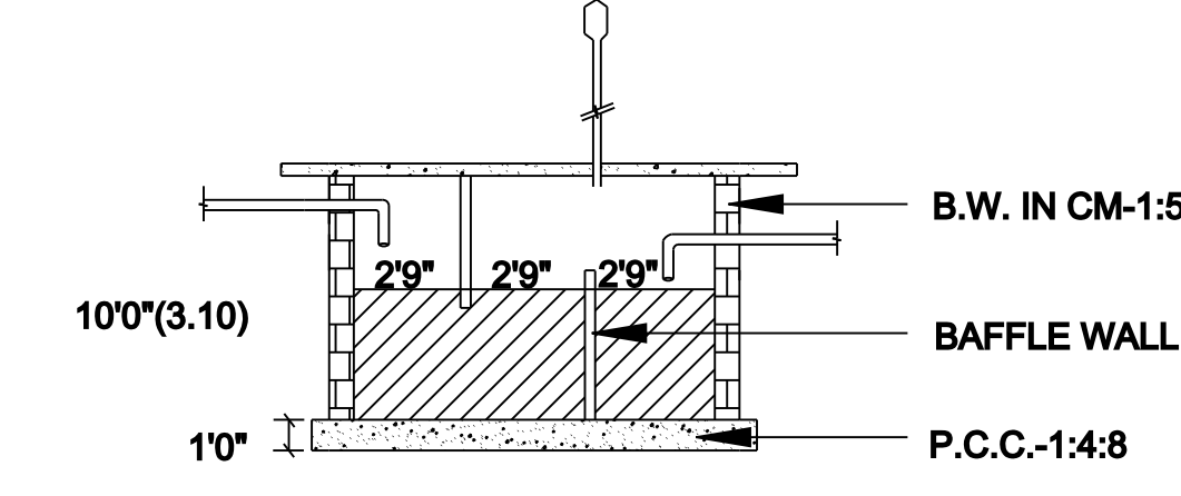
SEPTIC TANK SECTION-(XY)
