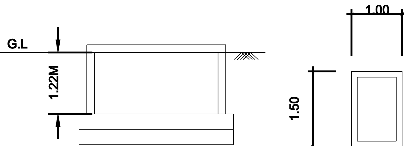
RWH_CAPACITY_L=2000LTRS
